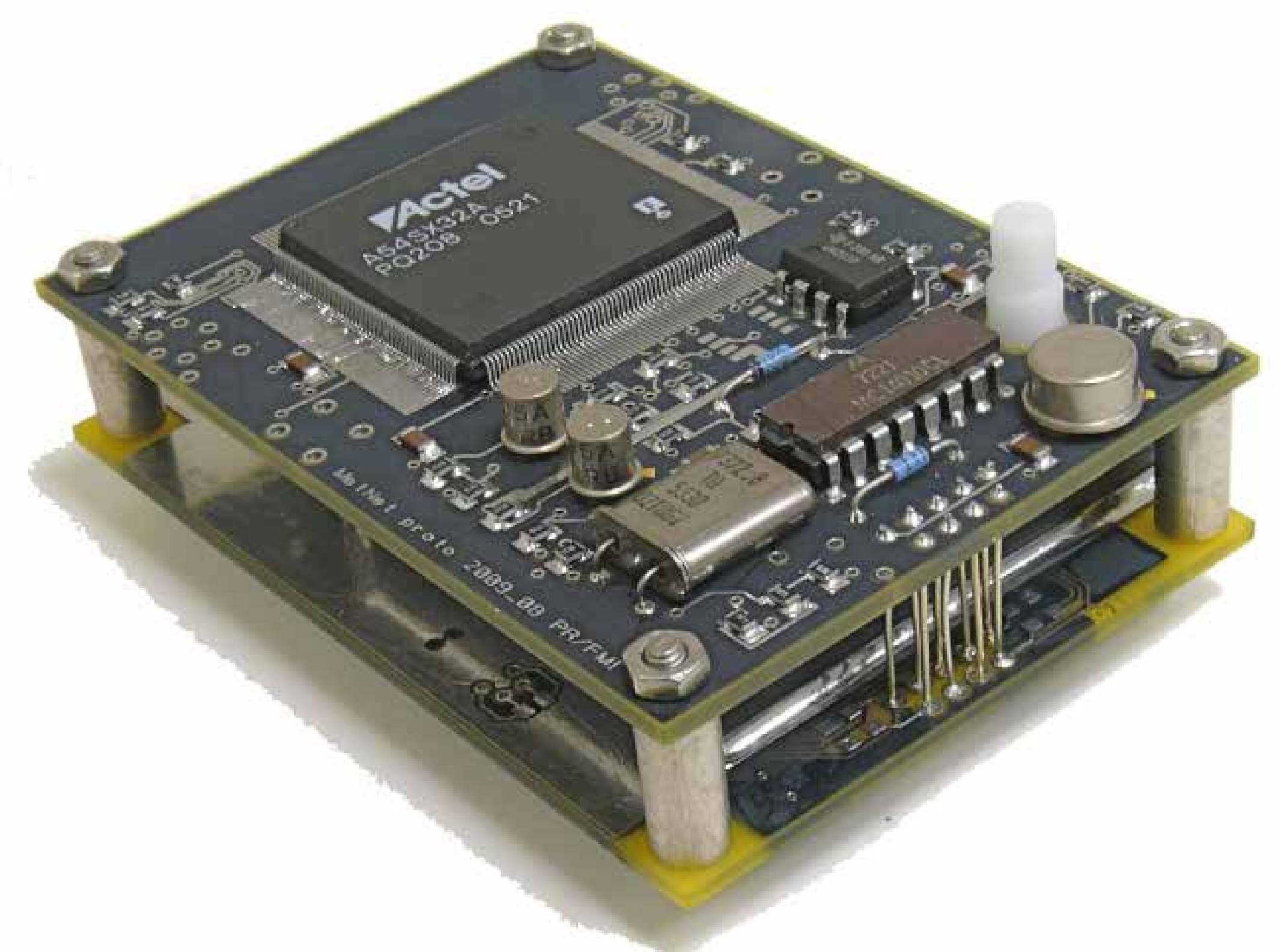
MetNet Mission pressure device MetBaro. Photo: Markku Mäkelä /FMI.
