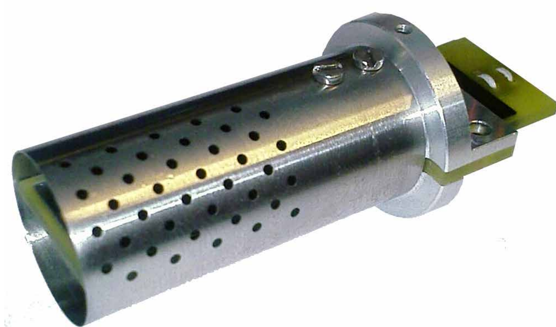
MetNet Mission humidity device MetHumi. Photo: Harri Haukka / FMI.
