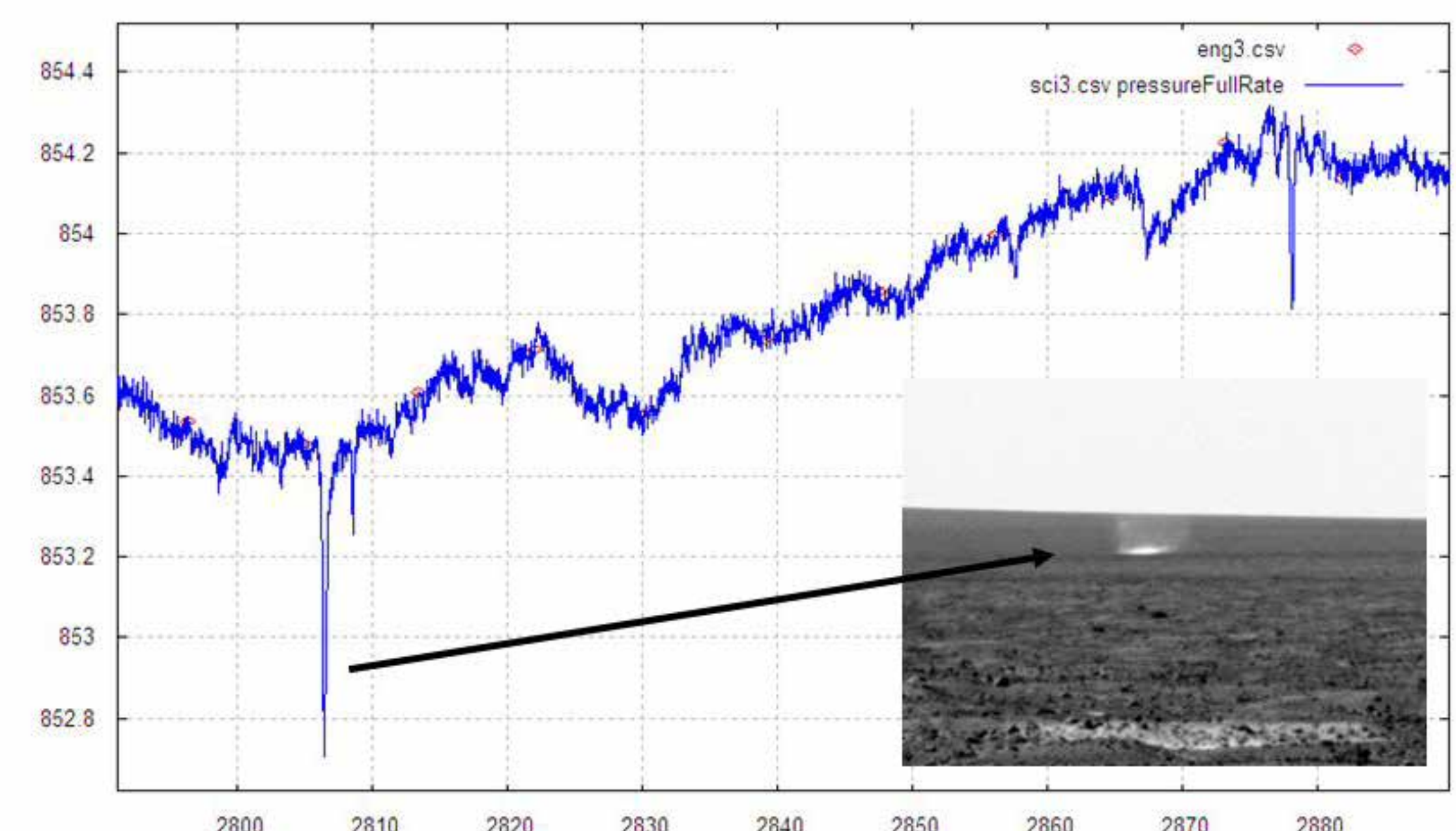
Pressure drops caused by dust devils detected by the FMI Phoenix Pressure device in Autumn 2008. Photo: NASA.
