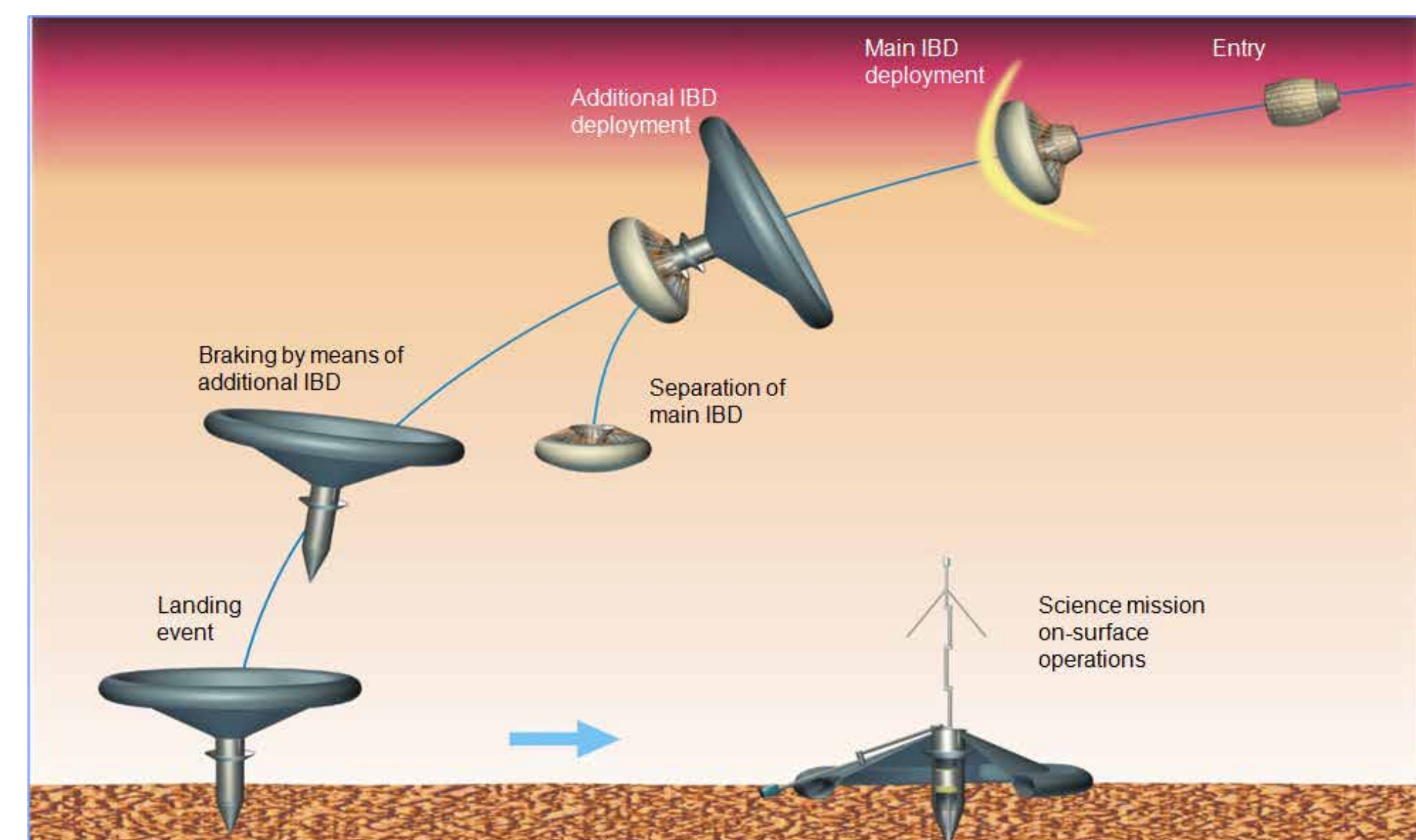
MetNet lander landing scheme. Picture: FMI.
